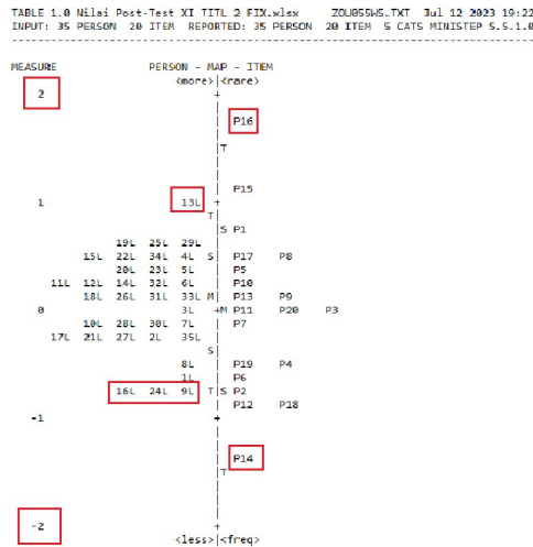
Gambar 6. Wright Map
