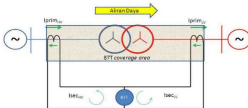
Gambar 1. Rele Diferensial Keadaan Arus Normal
