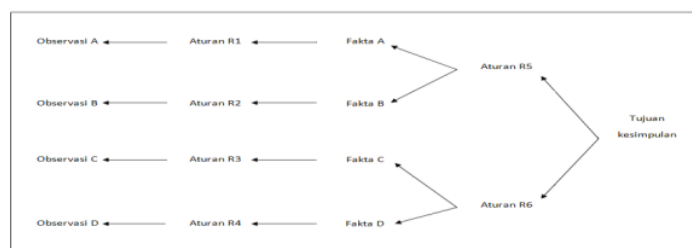
Gambar 2. Proses Backward Chaining
