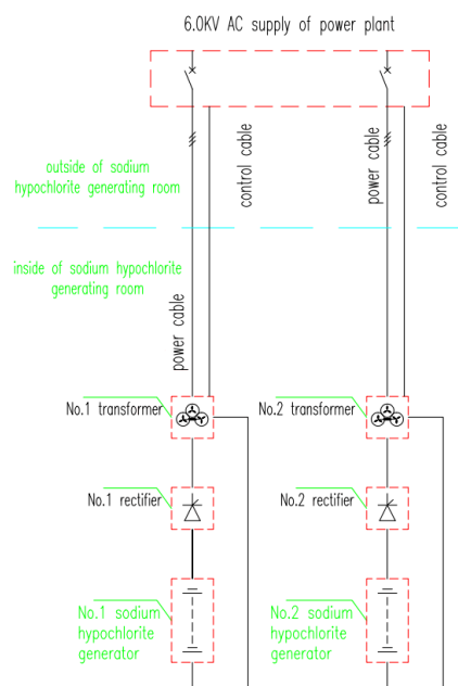
Gambar 5. Wiring Diagram Elektrolizer
