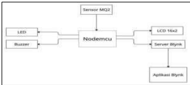
Gambar 1 Diagram Blok
