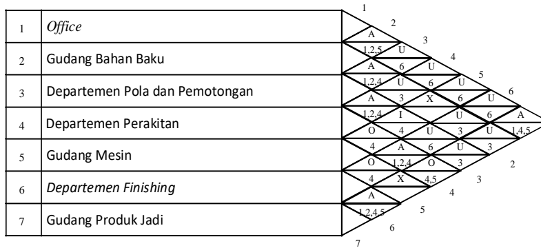
Gambar 3. Activity Relationship Chart (ARC)
