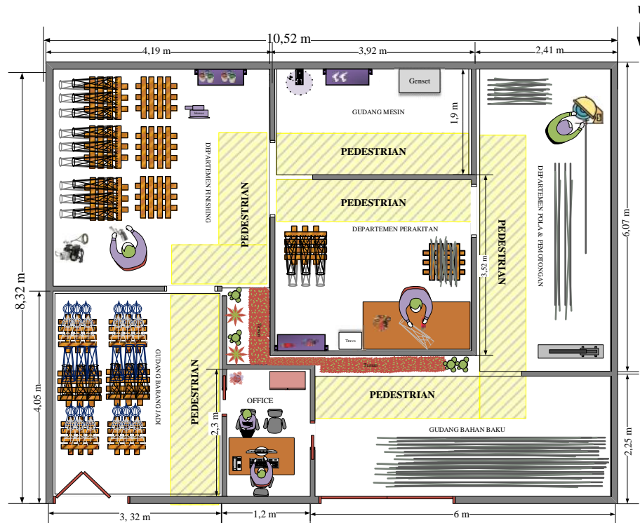
Gambar 5 Layout Usulan
